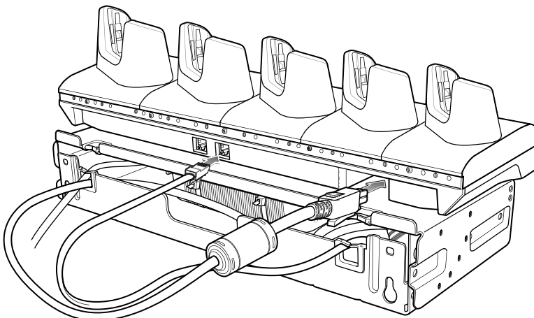
Figure 47 Connect Cables
