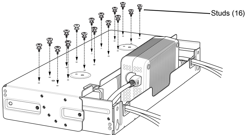
Figure 51 Install Studs
