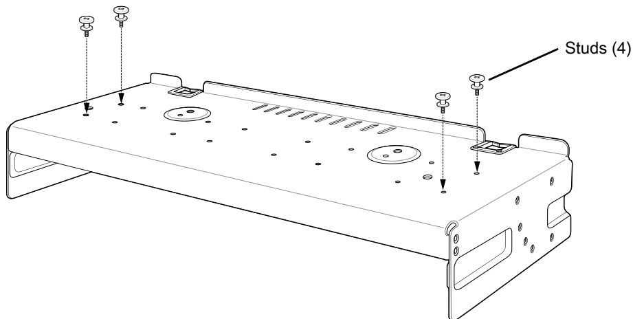
Figure 43 Install Studs
