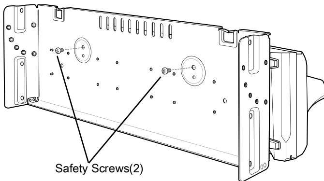
Figure 45 Secure Cradle
