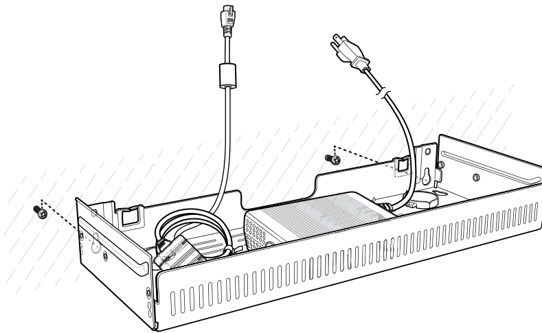
Figure 60 Horizontal Installation
