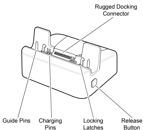
Figure 71 Rugged Communication and Charging Cradle - Rear View
