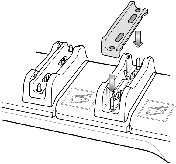
Figure 76 Install Insert in Slot
