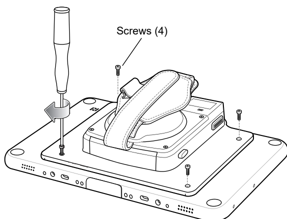
Figure 53 Secure Screws
