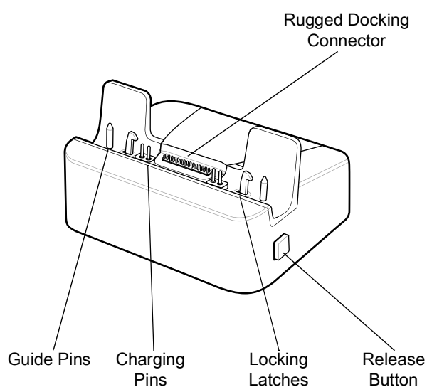
Figure 22 Rugged Communication and Charging Cradle - Rear View
