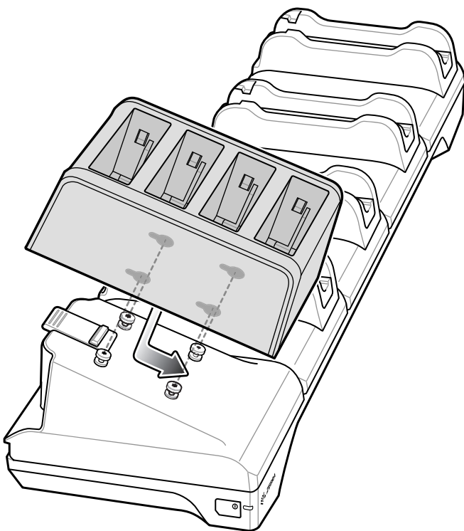
Figure 31 Align Battery Charger on Adapter
