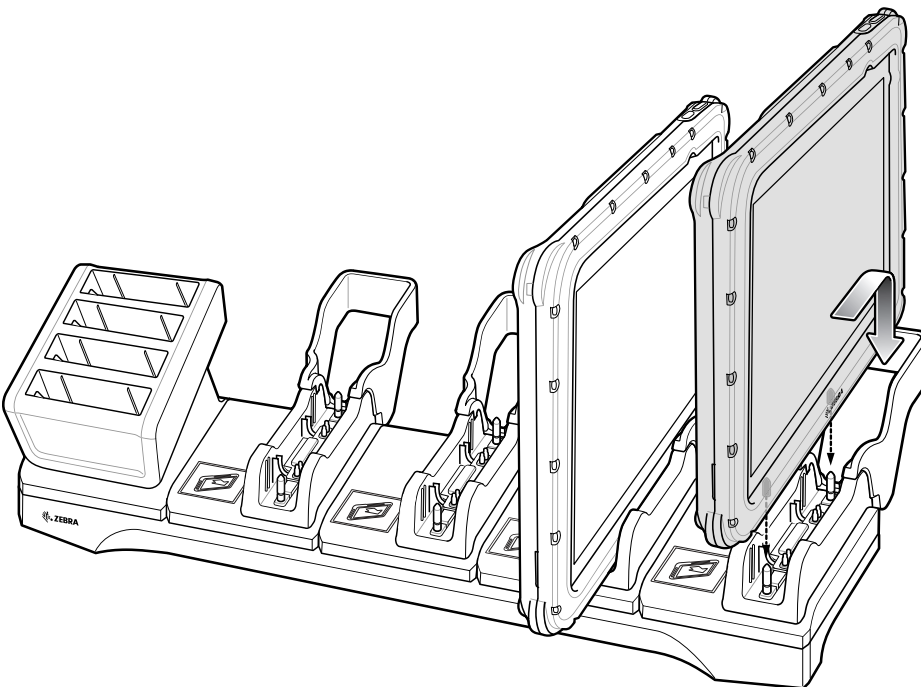
Figure 34 Insert device with Rugged Frame into Slot
