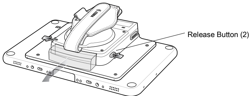
Figure 39 Remove Dummy Battery Insert
