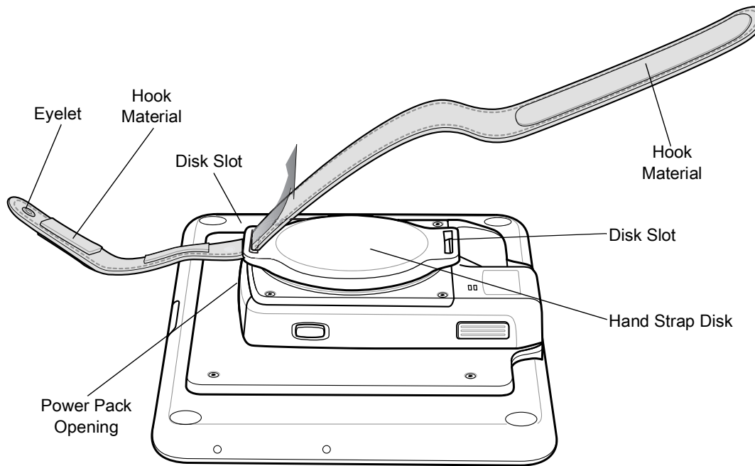
Figure 57 Feed New Strap
