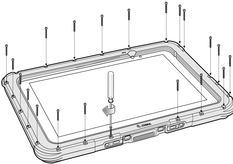
Figure 48 Secure 10" Rugged Frame
