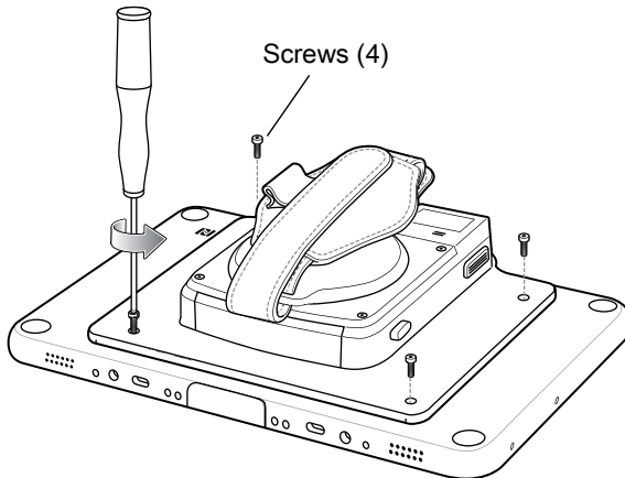
Figure 65 Remove Screws
