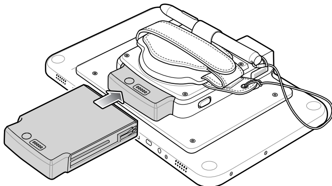
Figure 40 Install Power Pack
