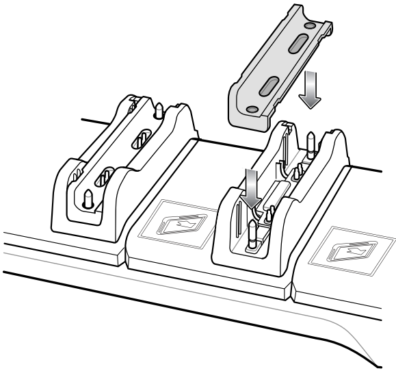
Figure 28 Install Insert in Slot
