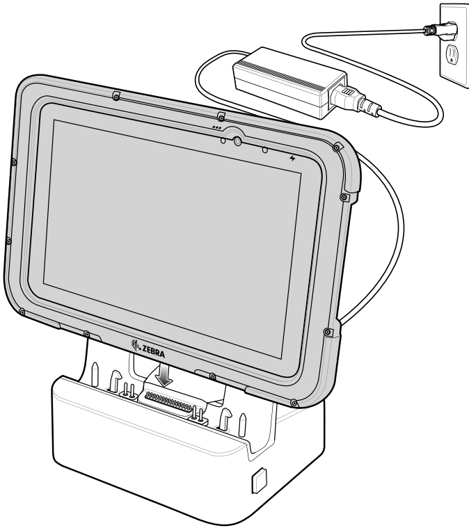
Figure 25 Insert Rugged Frame device and IO Adapter into Rugged Communication and Charging Cradle
