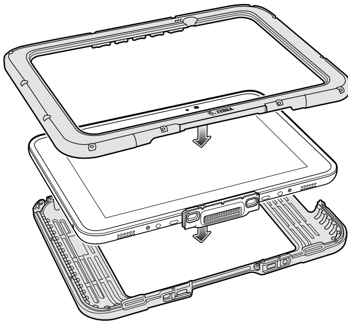
Figure 46 Protective Boot Assembly
