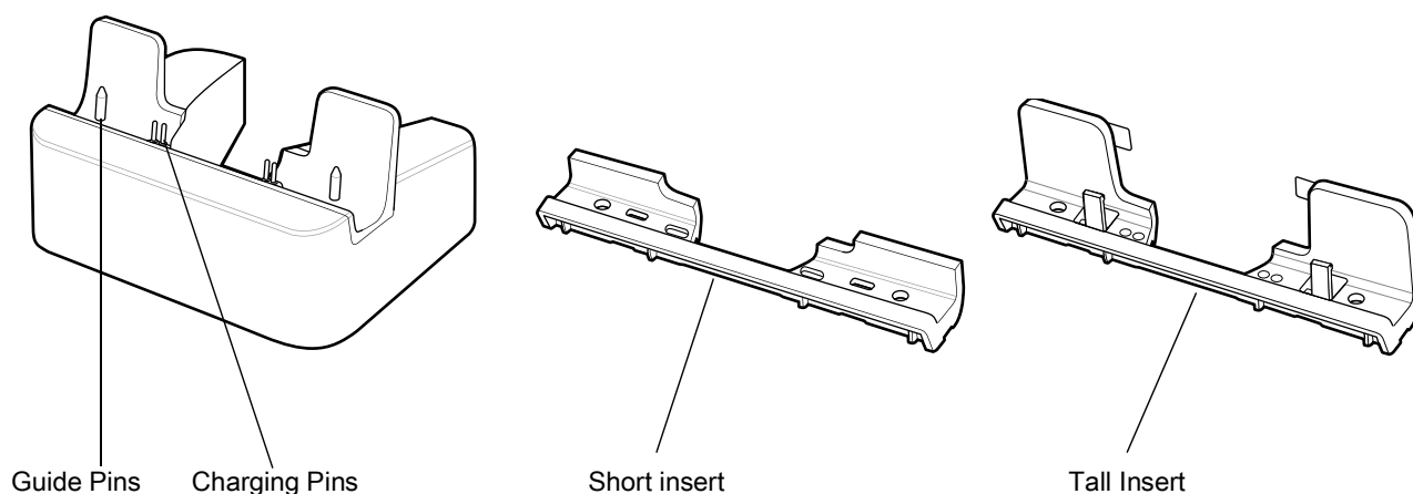
Figure 9 Charge Only Cradle - Front View
