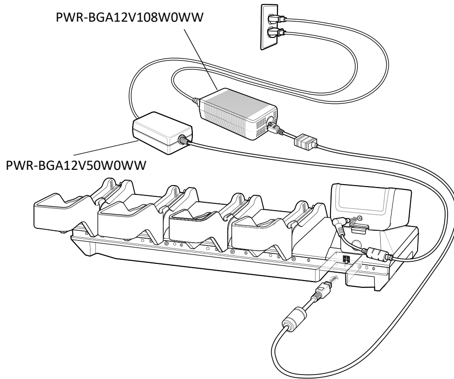
Figure 32 Power Setup with Optional Charger
