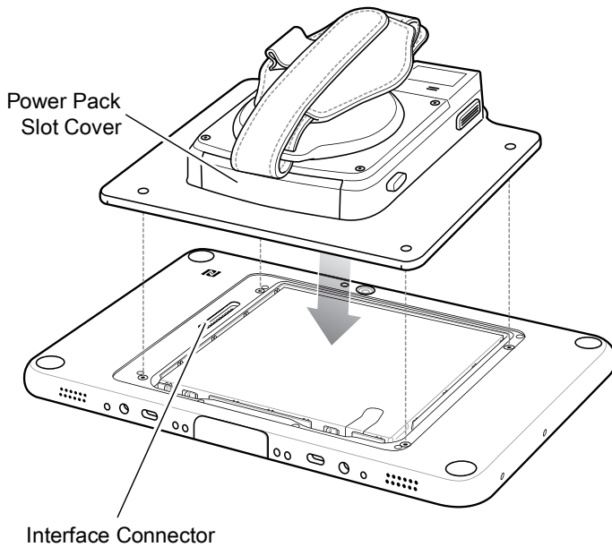
Figure 51 Align Expansion Back with 8" Configuration
