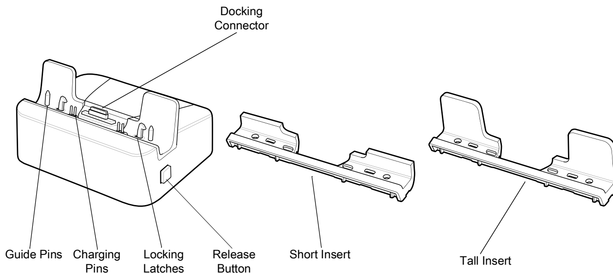
Figure 15 Communication and Charging Cradle - Front View
