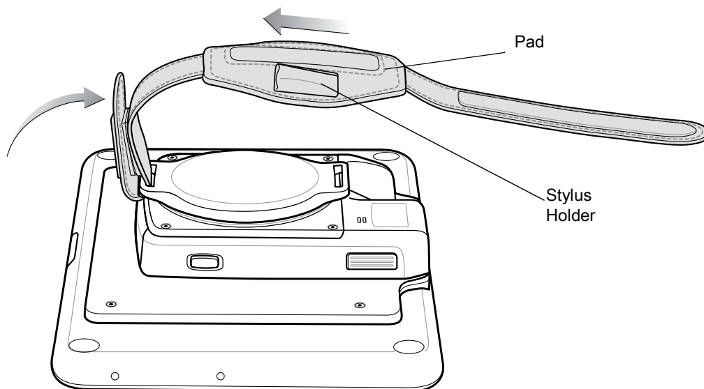
Figure 58 Secure Eyelet End
