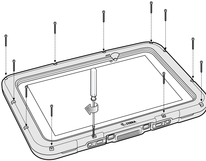
Figure 48 Secure 10" Rugged Frame
