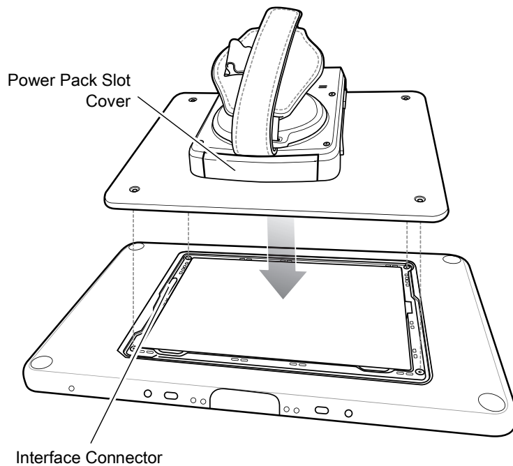
Figure 52 Align Expansion Back with 8" Configuration
