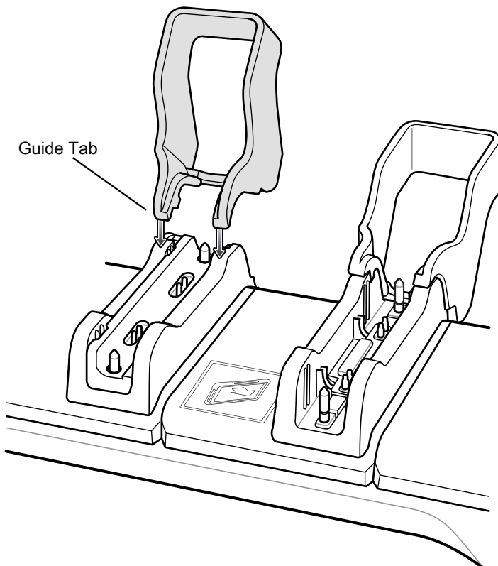
Figure 29 Align Guide with Slot
